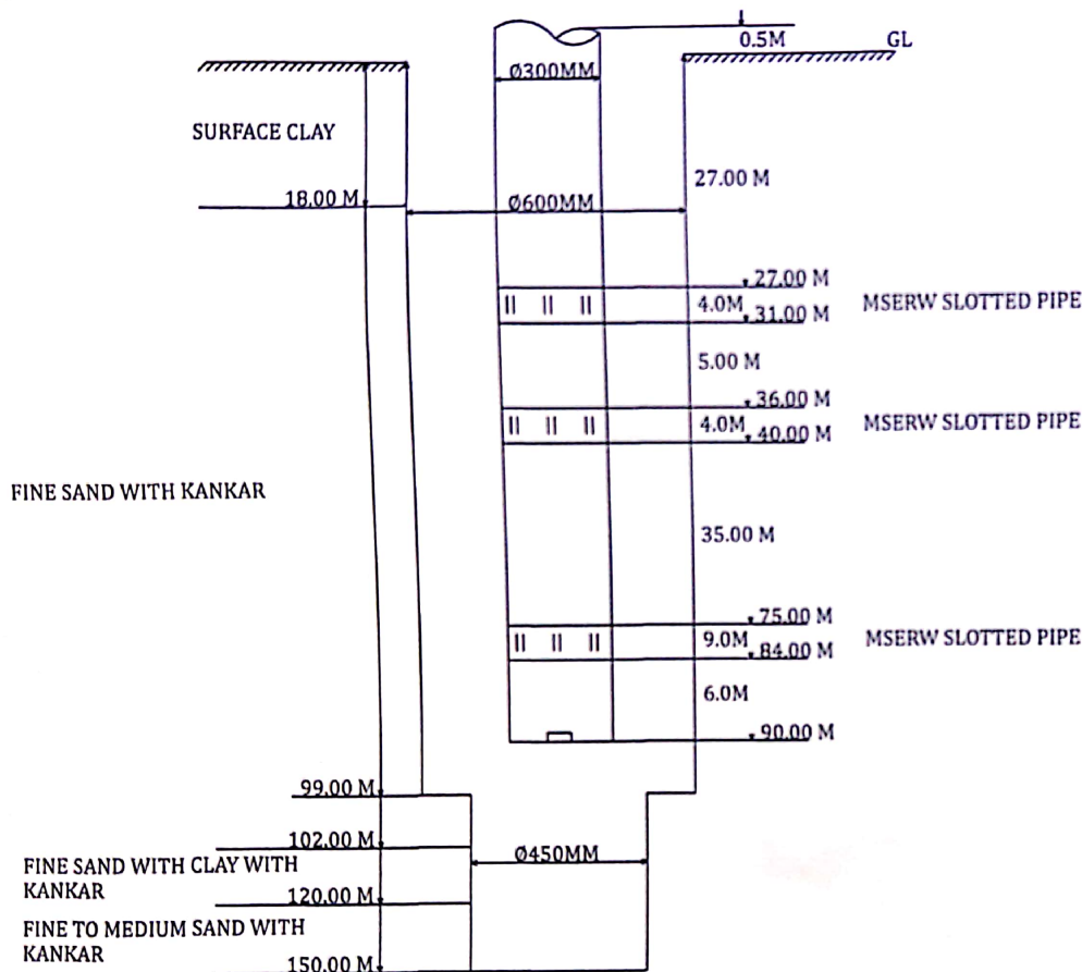
(A) PROPOSED TUBE WELL ASSEMBLY LOWERING DETAILS
