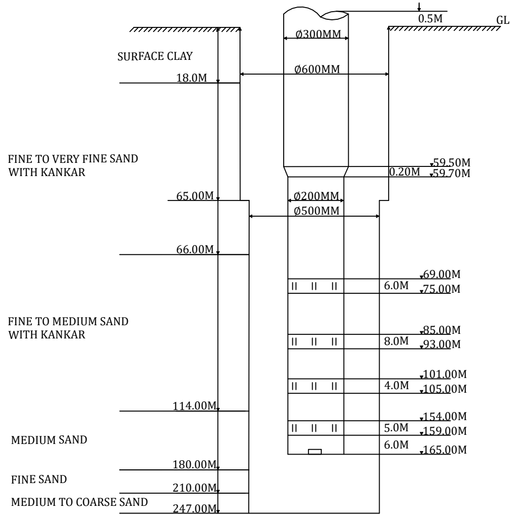
(A) ACTUAL TUBE WELL ASSEMBLE LOWERING DETAILS
