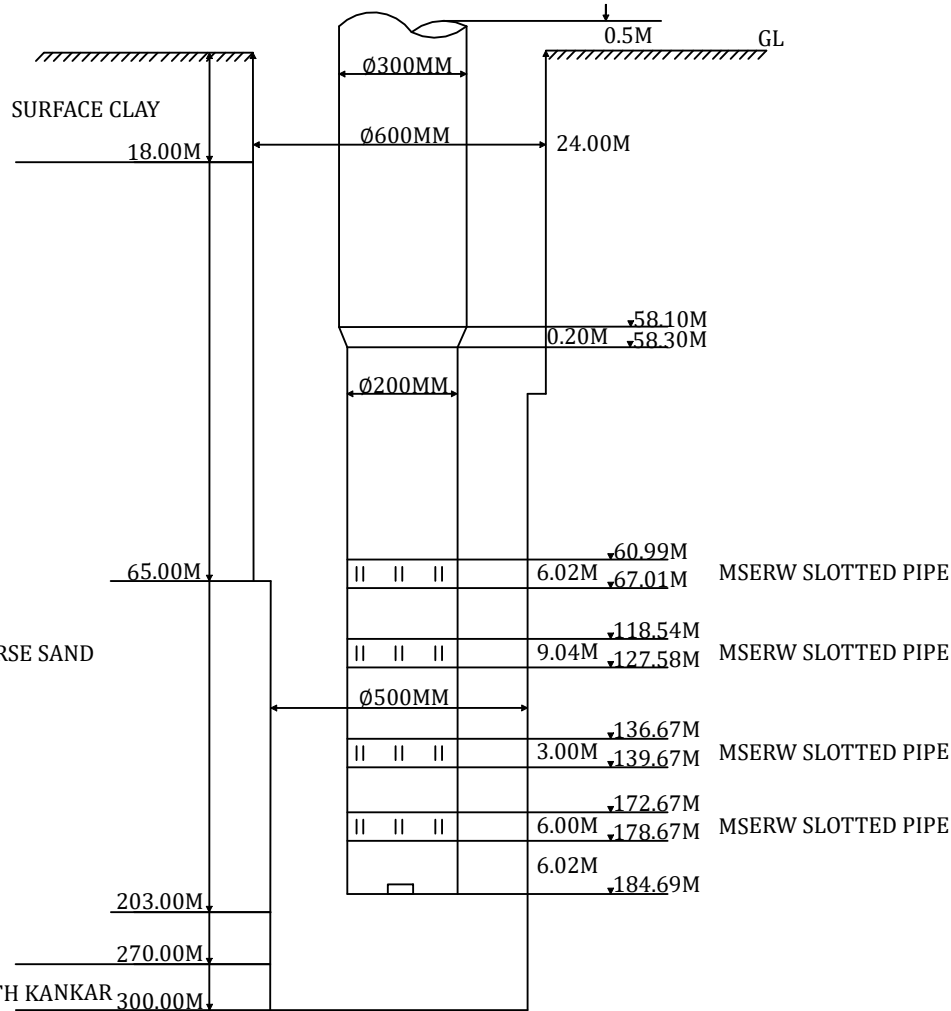
(A) PROPOSED TUBE WELL ASSEMBLY LOWERING DETAILS
