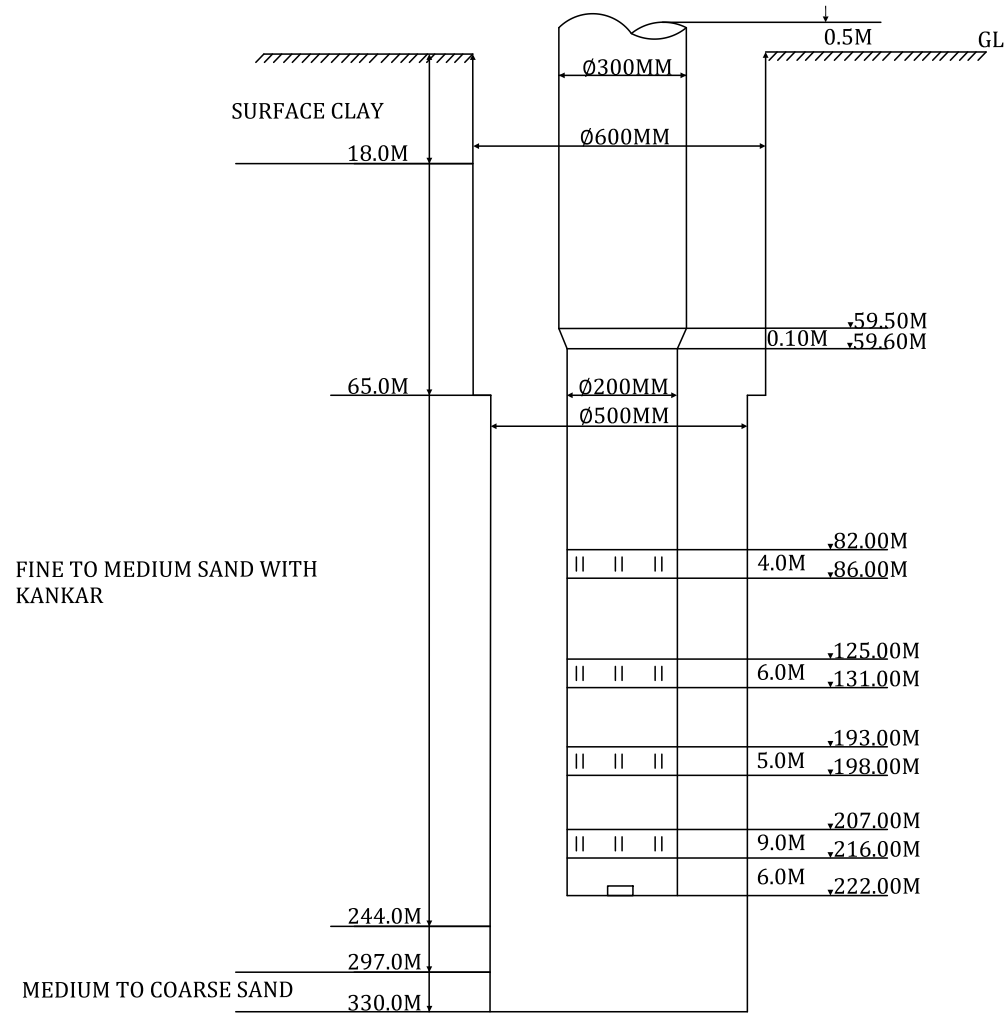
(A) PROPOSED TUBE WELL ASSEMBLE LOWERING DETAILS
