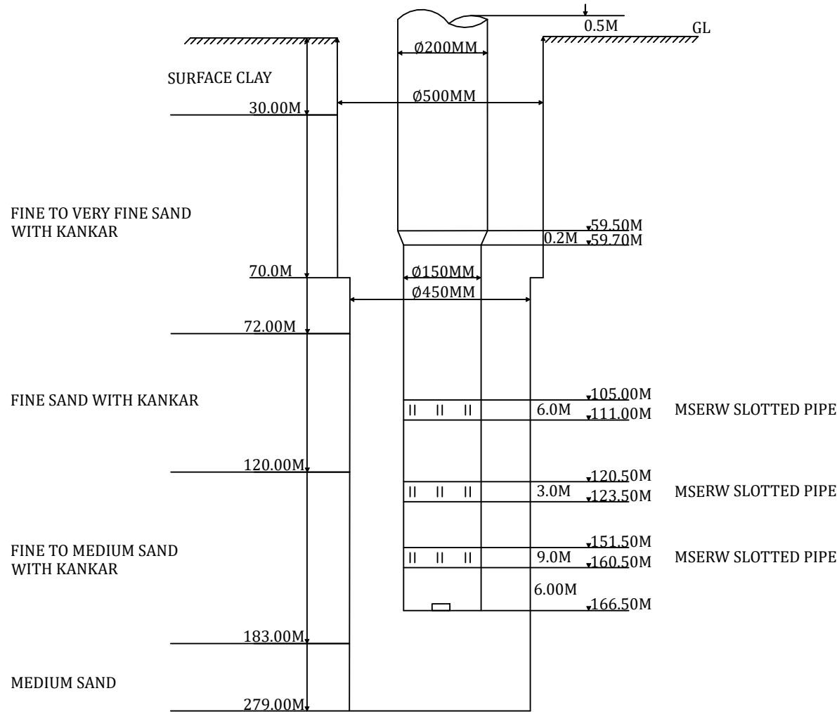
(A) ACTUAL TUBE WELL ASSEMBLE LOWERING DETAILS
