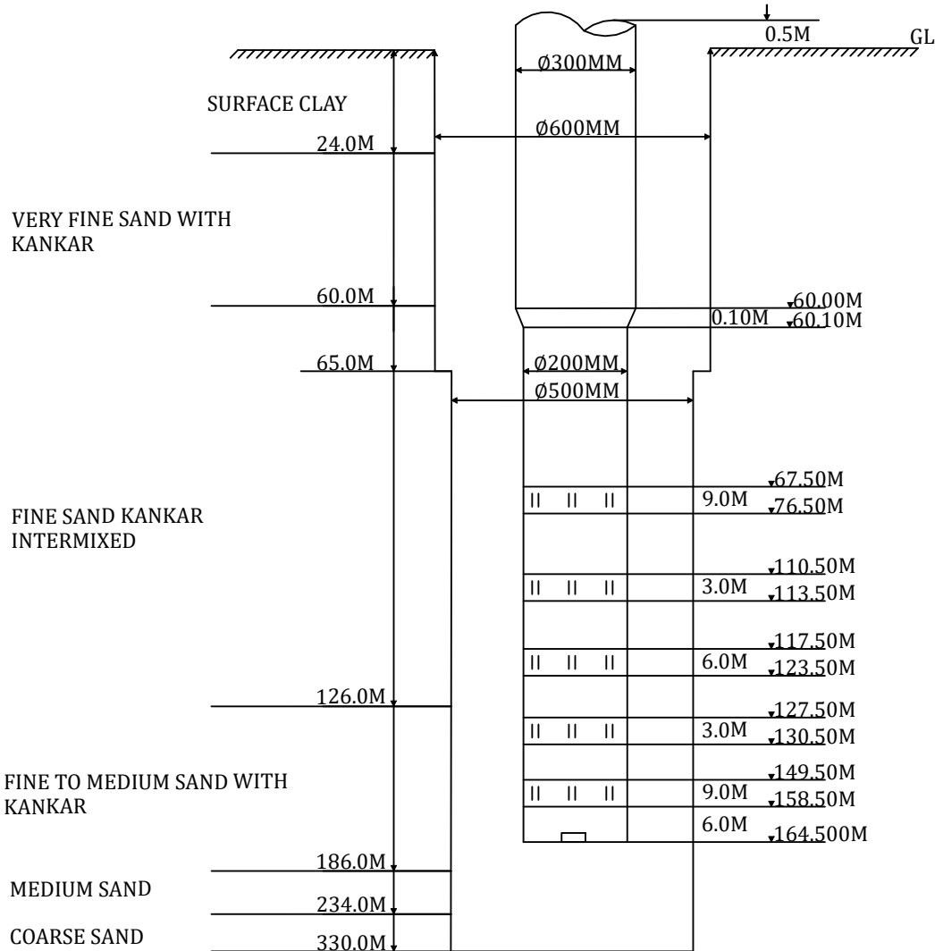
(A) PROPOSED TUBE WELL ASSEMBLY LOWERING DETAILS
