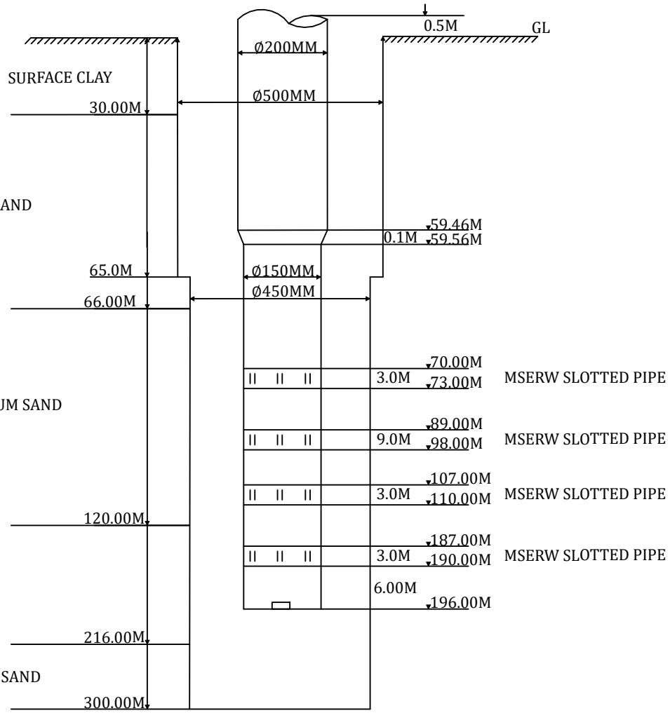
(A) ACTUAL TUBE WELL ASSEMBLY LOWERING DETAILS
