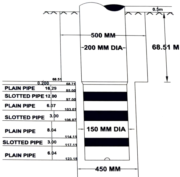
(A) ACTUAL TUBE WELL ASSEMBLY LOWERING DETAILS
