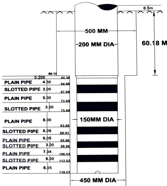
(A) ACTUAL TUBE WELL ASSEMBLY LOWERING DETAILS
